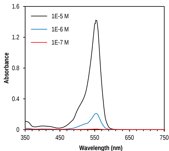
Figure (3) Absorption spectra of Rhodamine B dye dissolved in water at molar concentrations of 1 \times 10^{-5} , 1 \times 10^{-6} , and 1 \times 10^{-7}
