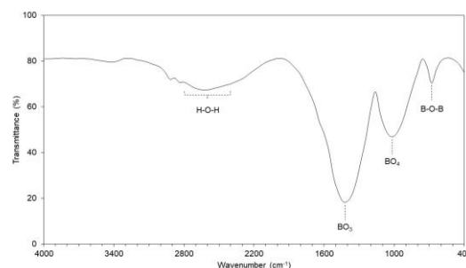
Fig. (2) FTIR spectra of the samples prepared in this work using Ar:O 2 mixing ratio of 4:1 and deposition time of 30 s
