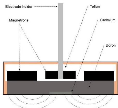
Fig. (1) Configuration of the B and Cd targets and magnetron on the cathode
