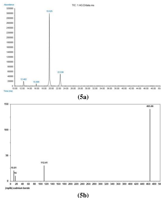
Fig. (5) GC spectrum (a) and MS analysis (b) of the sample prepared using gas mixture of 4:1 and deposition time of 30 s
