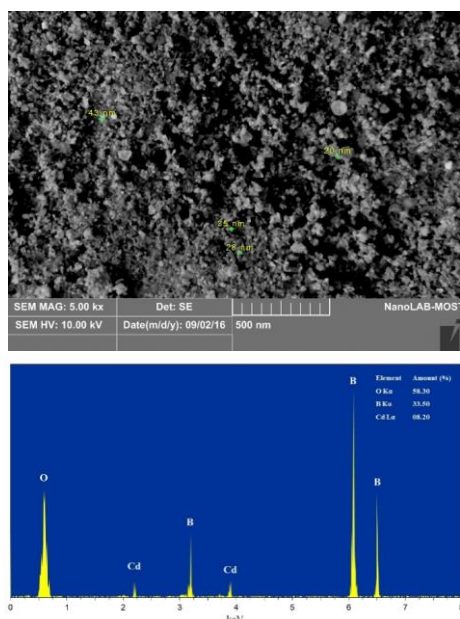
Fig. (4) SEM and EDS results of the cadmium borate sample prepared using gas mixture of 4:1 and deposition time of 30 s
