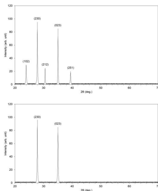
Fig. (3) Simulated XRD patterns of the cadmium borate samples prepared in this work using Ar:O 2 mixing ratio of 1:1 and deposition time of 60 s (upper) and 4:1 and 30 s (lower)
